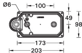
MOUNTING DETAIL
