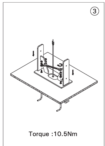
MOUNTING DETAIL
