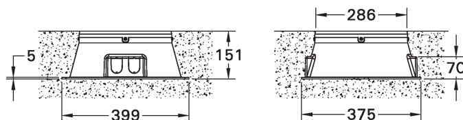
FLAT FRAME KI-60781, KI-60785
