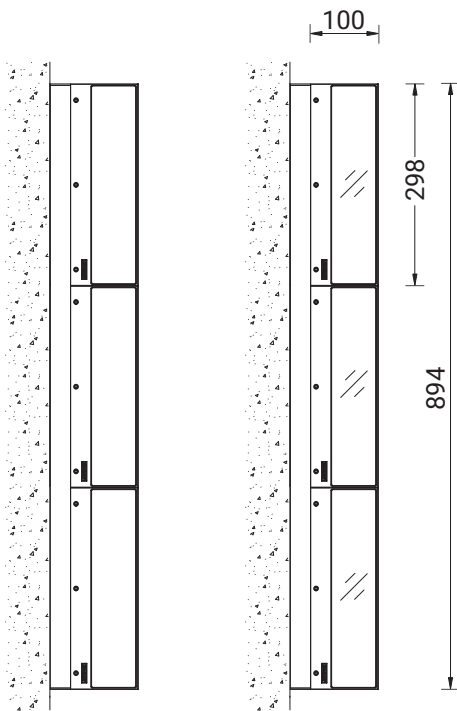
Top view
