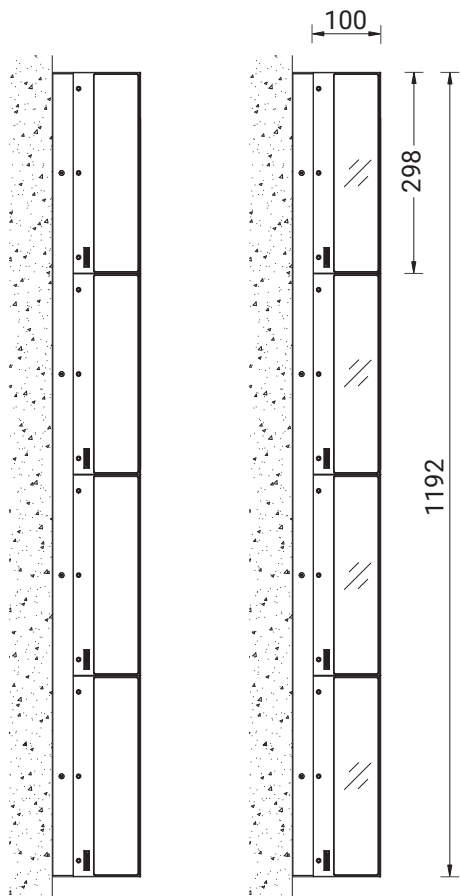
Top view
