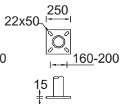
Steel post Mounting detail
