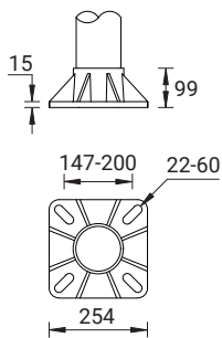
Mounting detail
