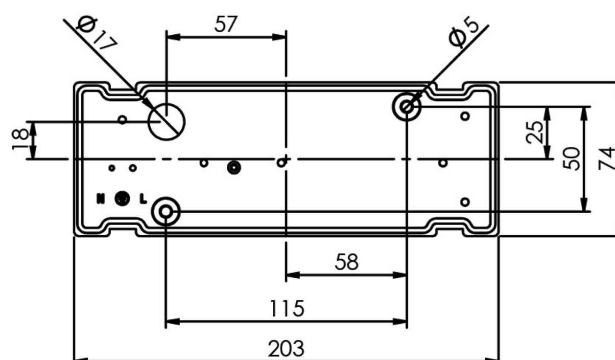
MOUNTING DETAIL
