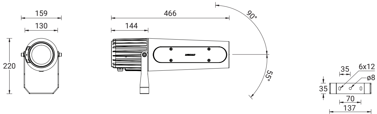
Mounting detail
