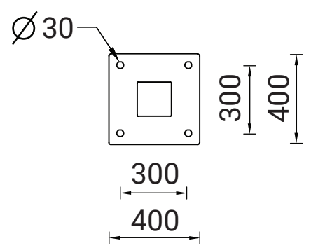
Mounting detail
