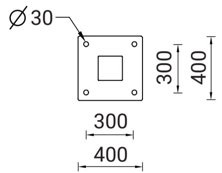
Mounting detail
