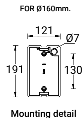
Mounting detail
