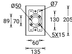
Mounting detail
