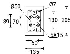
Mounting detail
