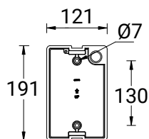
Mounting detail
