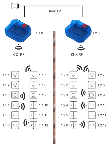
KNX RF/TP Coupler as line coupler
