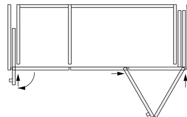
Hawa Folding Concepta III 25 Pull, right with Hawa Concepta III 35 Pull, left
