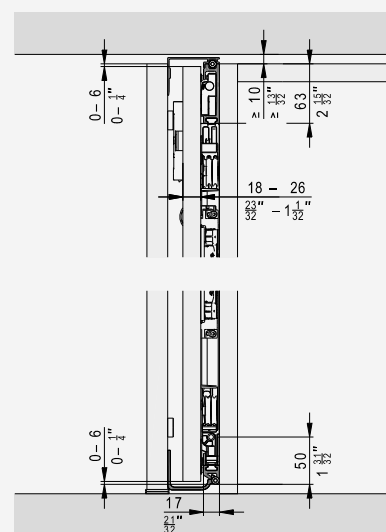
Overlay door without base
