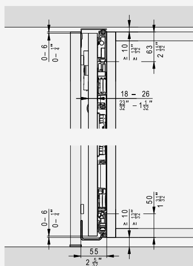
Door striking against the top and bottom cabinet sections
