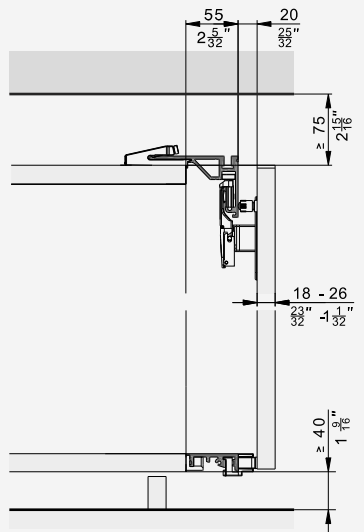
Overlay door with base profile in conjunction with Hawa Concepta III 25/35 Pull
