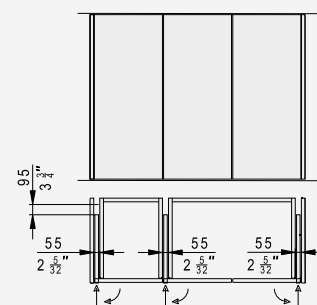
Overlay door without base
