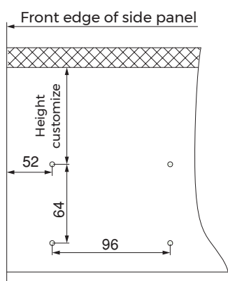
Left installing hole position
