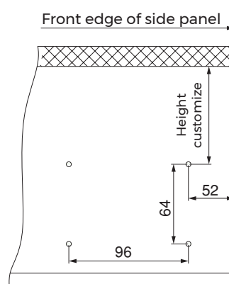
Right installing hole position
