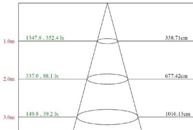
Max , Ave Beam angle of C120 plane 118.88
