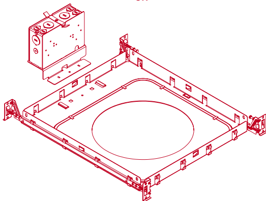
NEW CONSTRUCTION | PLASTER FRAME | L
