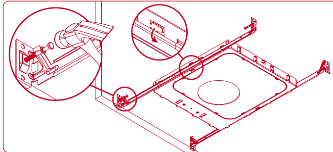
NEW CONSTRUCTION PLASTERFRAME | S
