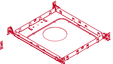
NEW CONSTRUCTION PLASTERFRAME | L
