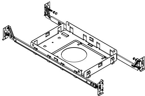
NEW CONSTRUCTION PLASTER FRAME | S
