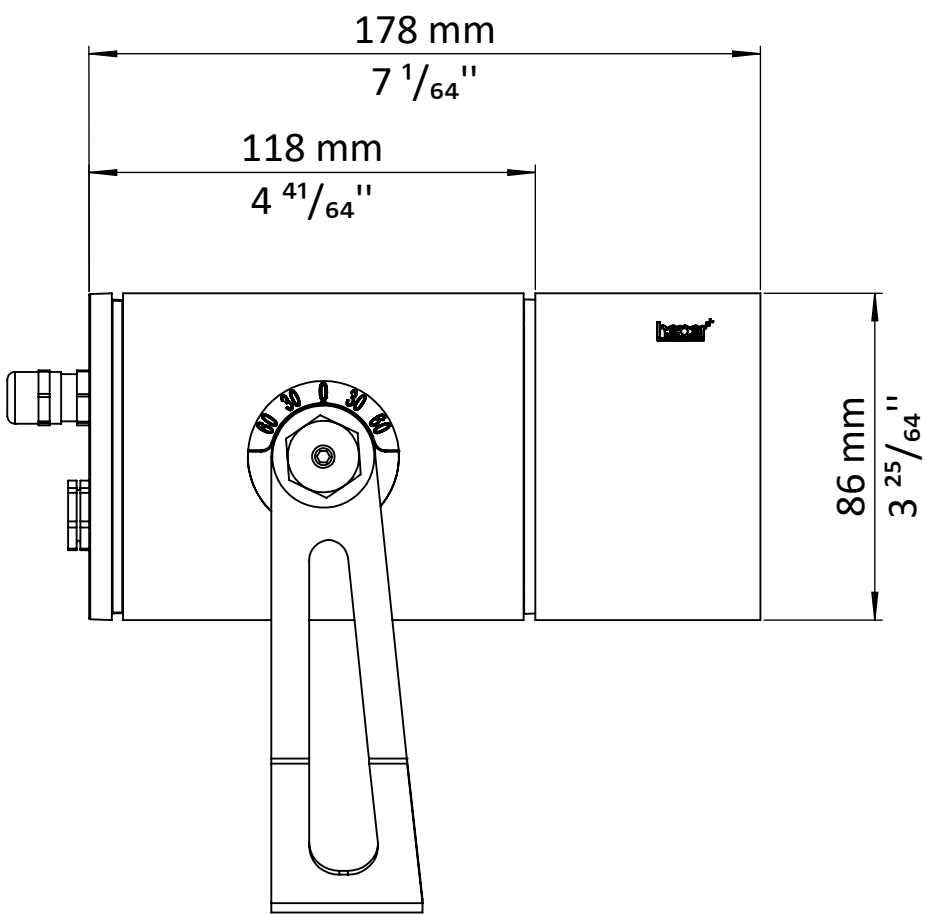
VEGA S (ON/OFF)
