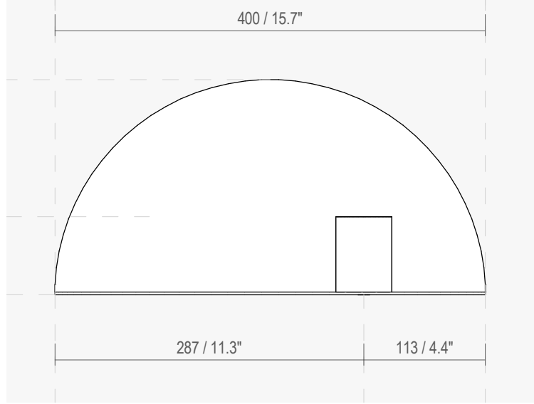
Fixing Dimensions
