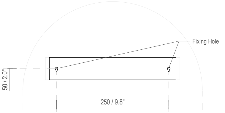
Fixing Dimensions
