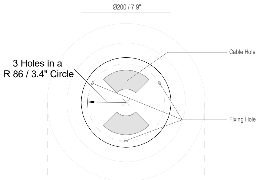
Fixing Dimensions
