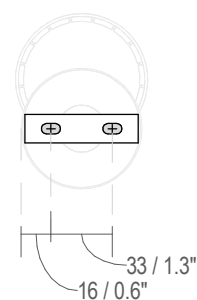
Fixing Dimensions
