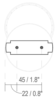
Fixing Dimensions
