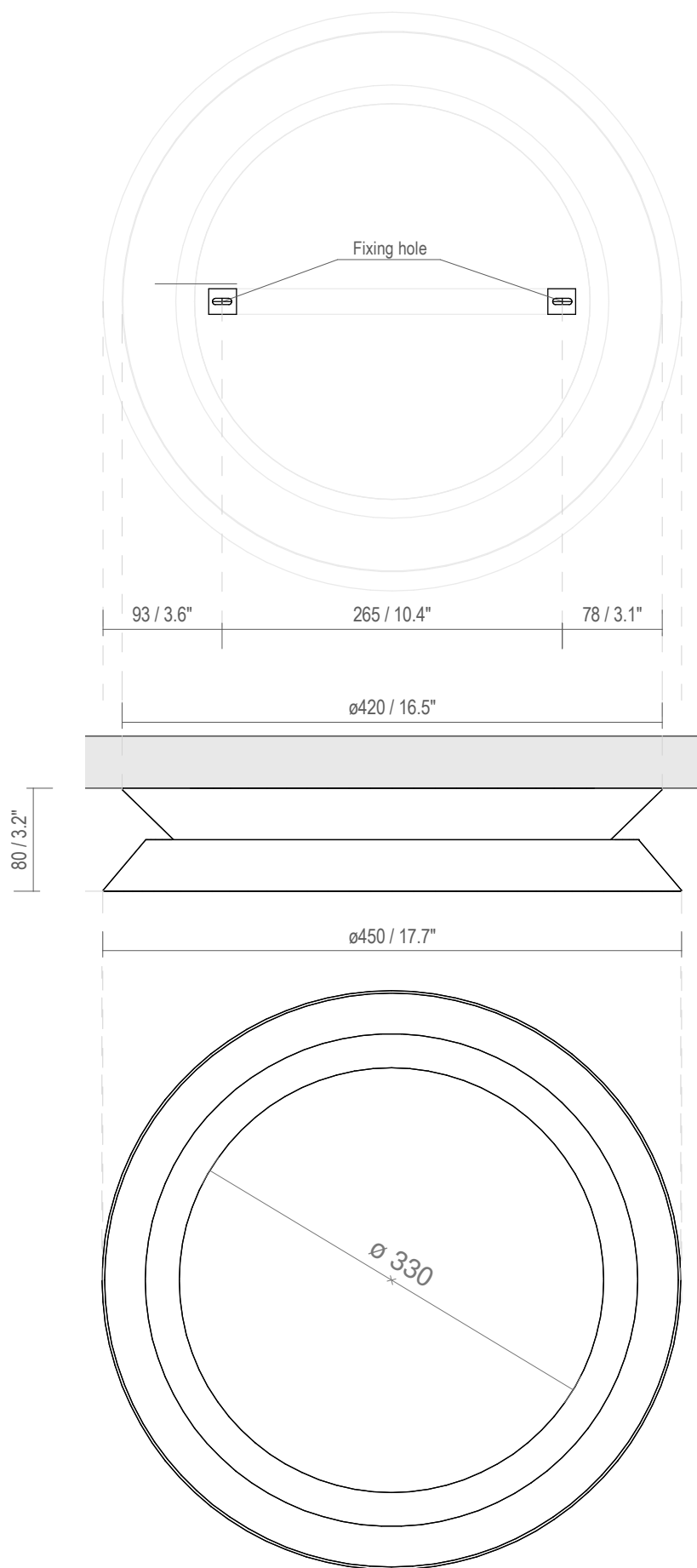
Fixing Dimensions
