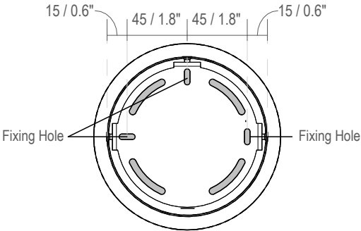
Fixing Dimensions
