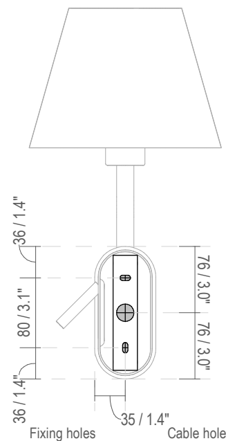
Fixing Dimensions
