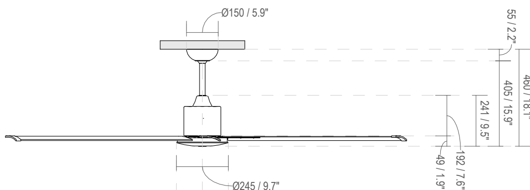
Fixing dimensions
