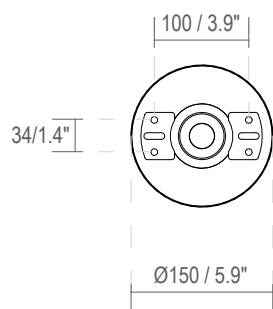
Fixing dimensions
