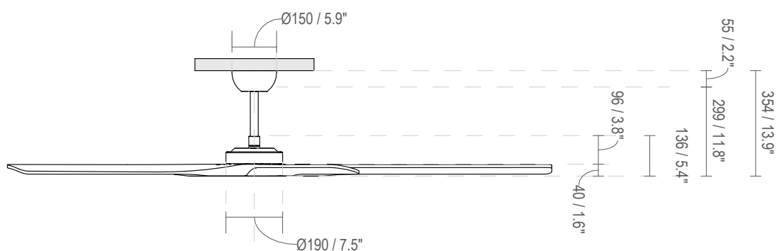
Fixing dimensions
