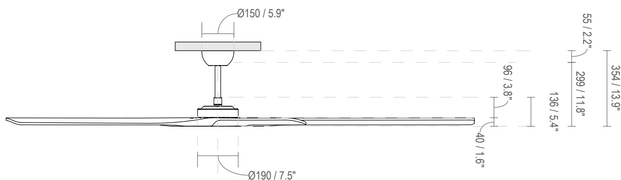
Fixing dimensions
