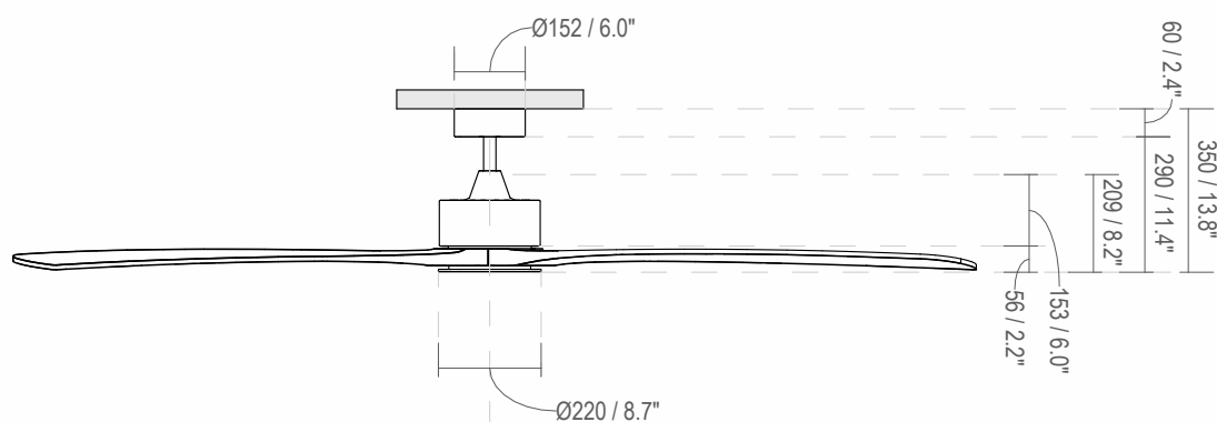
Fixing dimensions
