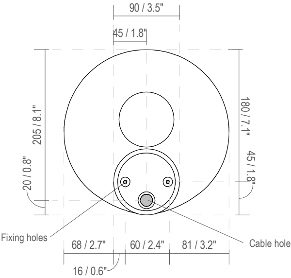
Fixing Dimensions
