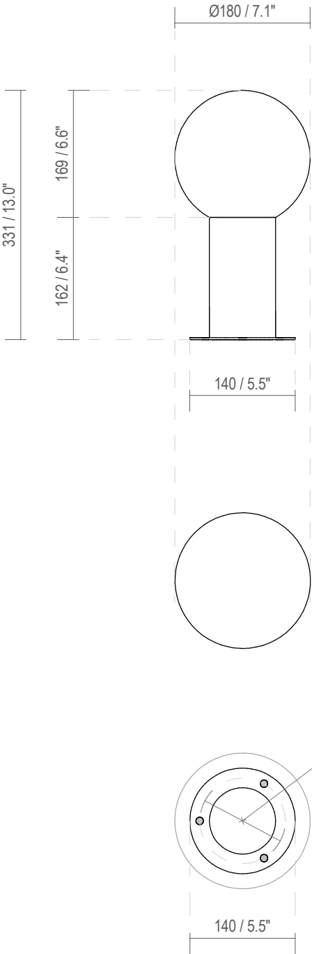
Fixing dimensions
