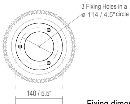
Fixing dimensions
