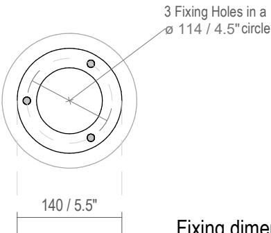
Fixing dimensions
