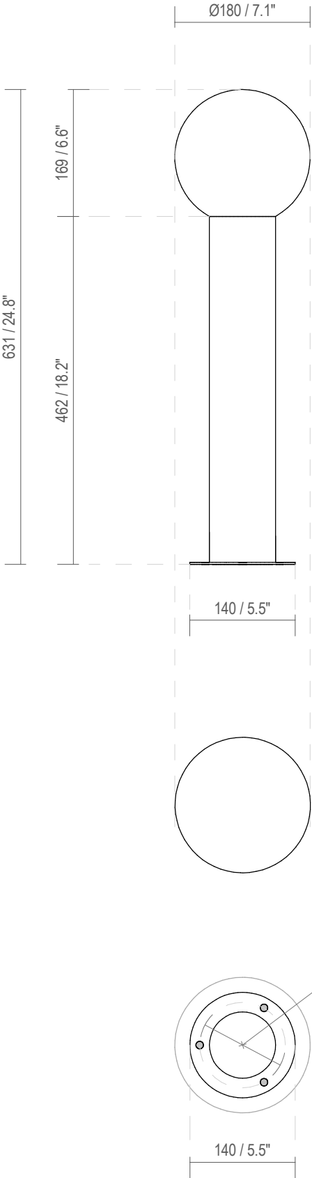
Fixing dimensions
