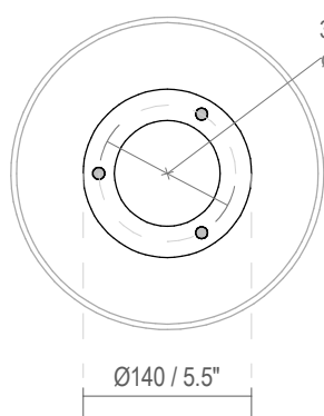
Fixing dimensions
