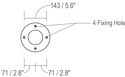
Fixing dimensions
