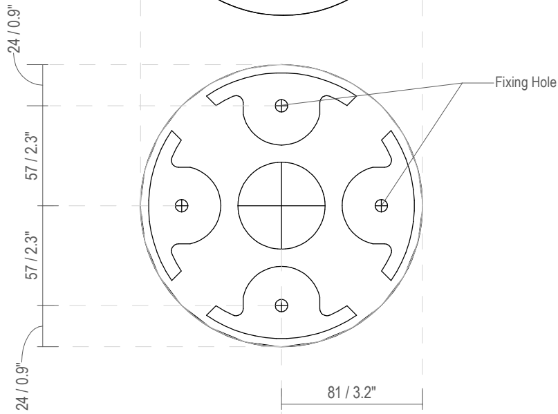
Fixing dimensions
