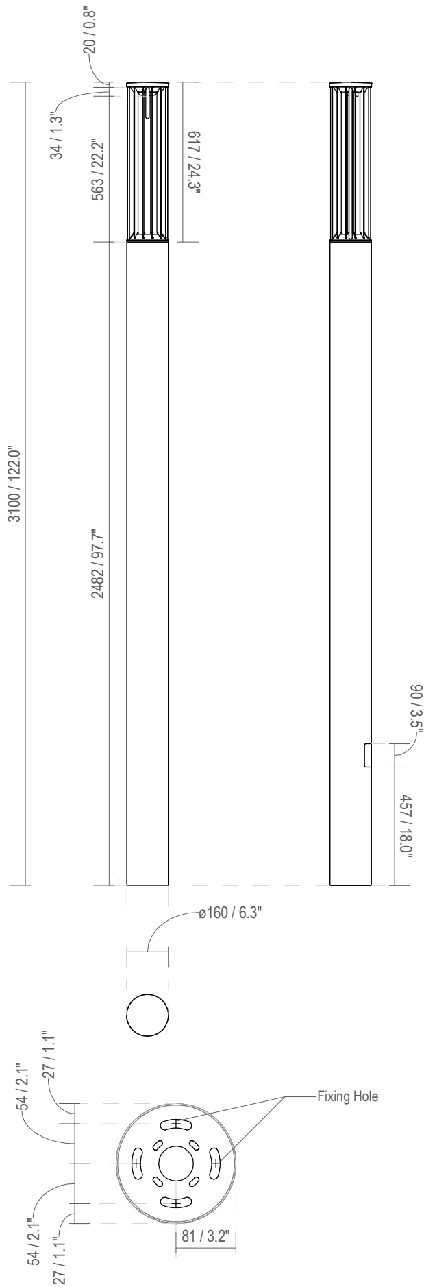
Fixing dimensions
