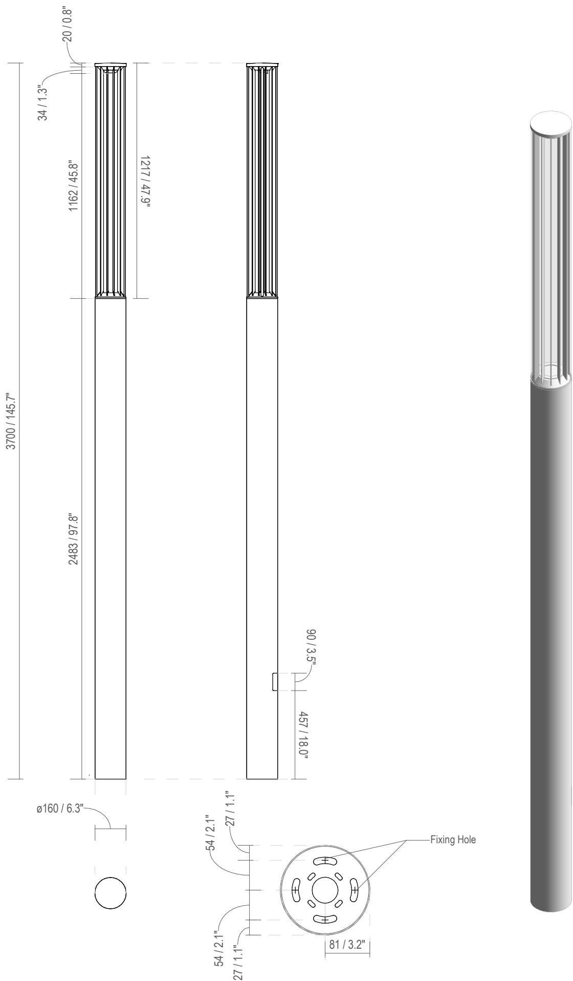
Fixing dimensions
