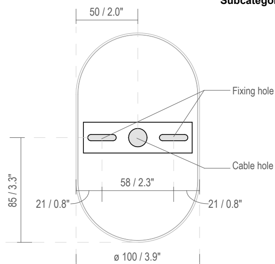
Fixing Dimensions
