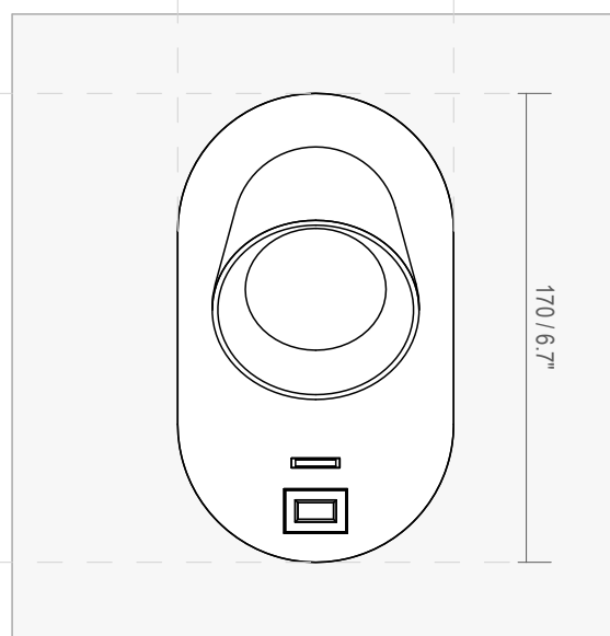
Fixing Dimensions
