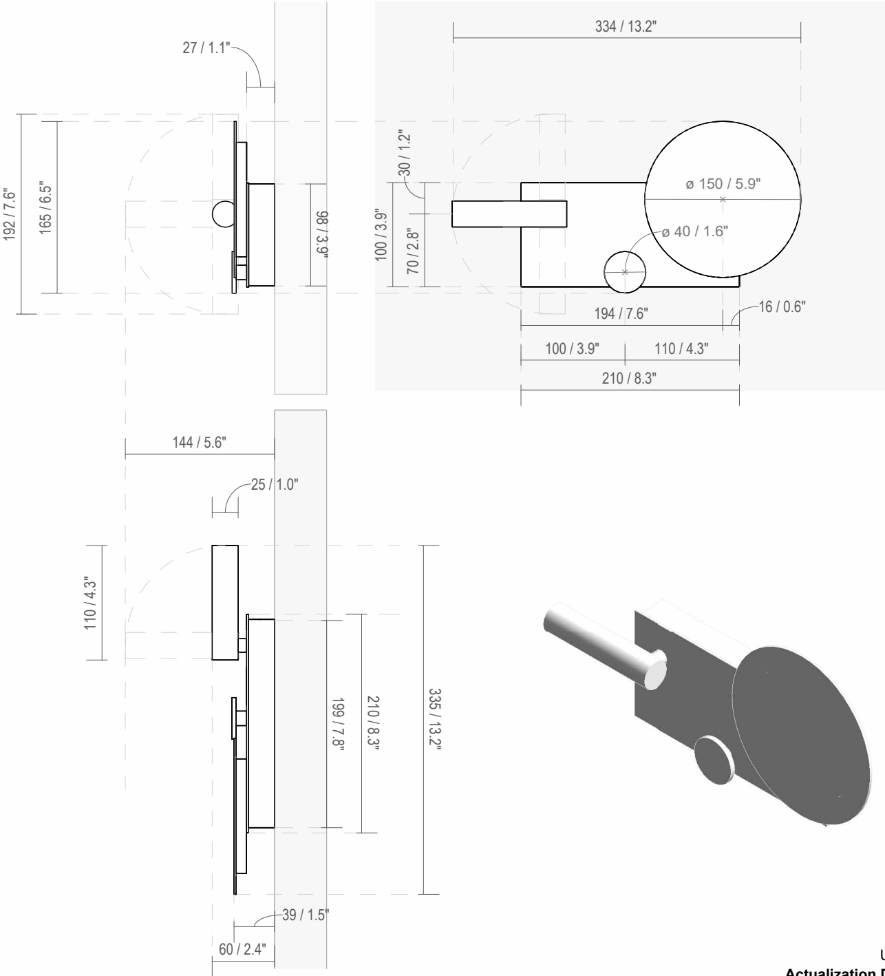
Fixing Dimensions
