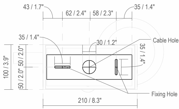
Fixing Dimensions
