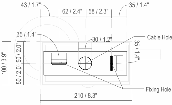
Fixing Dimensions
