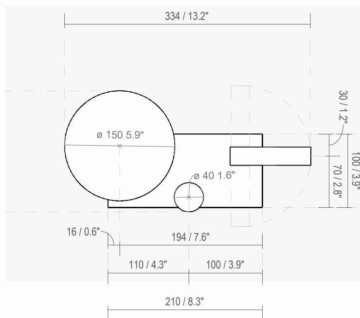
Fixing Dimensions
