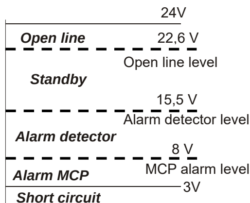
Figure 8: Zone Voltage thresholds.
