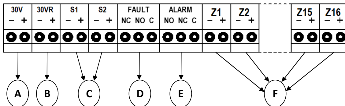
Figure 4: CPU Control panel connectors
