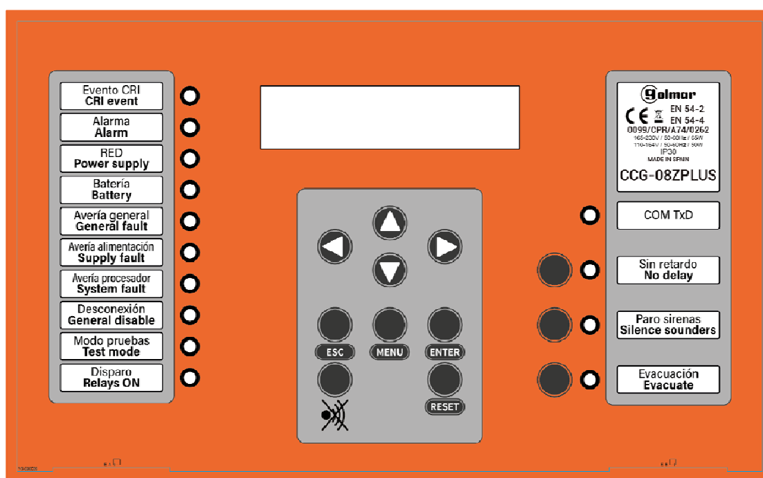
Figure 7: CCG-XXZPLUS control panel
