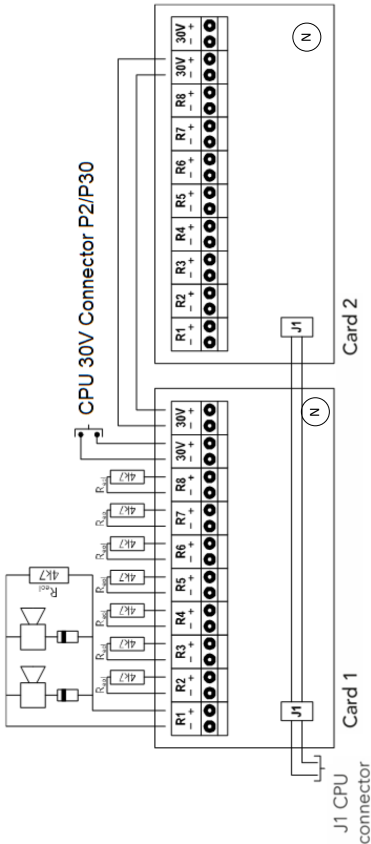
Figure 2: SRxx-PLUS card relay scheme connection
