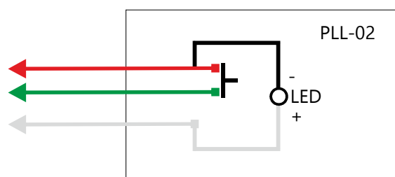
Internal scheme
