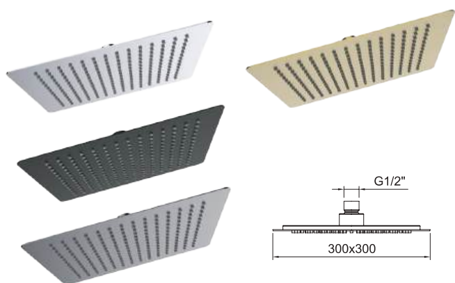
Douche de tête Slim Inox Air 300x300mm. Slim Inox Air head shower 300x300mm.
