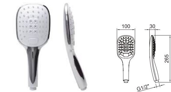
Douchette Style 100x120mm. Style shower handset 100x120mm.
