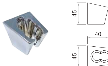
Support douchette fixe. Fix handset holder.
