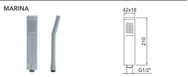
Douchette Marina. Marina shower handset.
