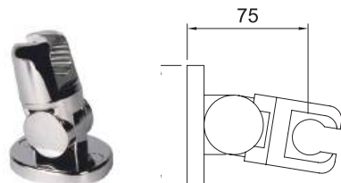
Support douchette orientable. Articulated handset holder.
