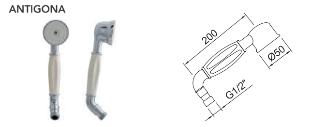
Douchette Antigona Ø50mm. Antigona shower handset Ø50mm.
