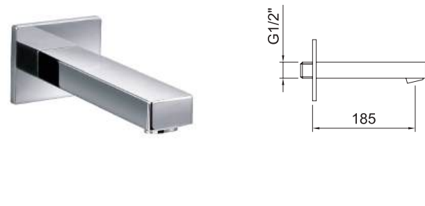
Caño mural Bimini. 185mm Bath spout Bimini. 185mm
