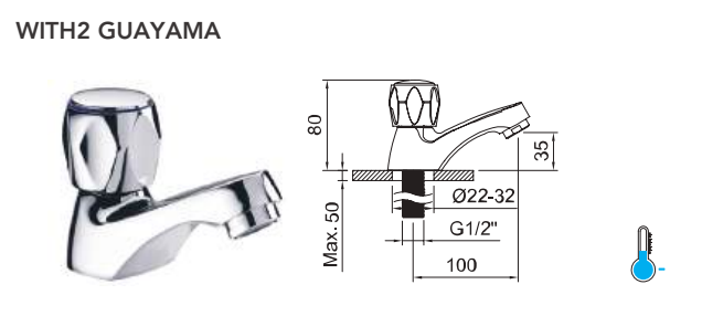
Grifo lavabo repisa 1/2" con aireador. Deck mounted basin tap 1/2" with aerator.
