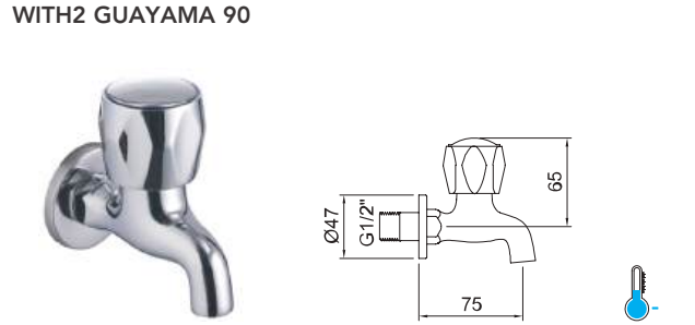
Grifo lavabo mural 1/2". Wall mounted basin tap 1/2".
