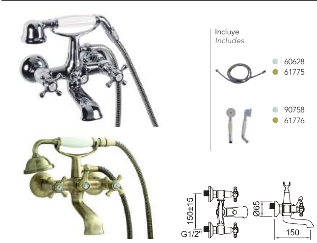
Baño-ducha bimando con inversor manual. Two-handed bath-shower mixer with diverter manual.
