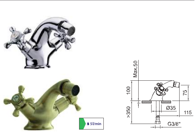
Bidé bimando con aireador a rótula y flexibles 3/8" >350mm. Two-handed bidet mixer with swivel aerator and flexible hoses 3/8" >350mm.
