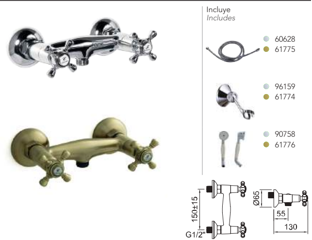
Ducha bimando. Two-handed shower mixer.
