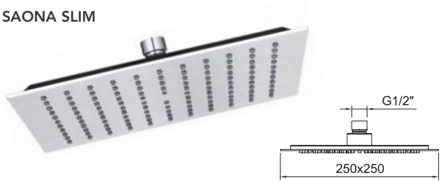
Rociador ducha Saona Slim 250x250mm. Saona Slim head shower 250x250mm.
