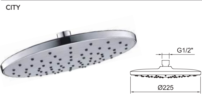
Rociador ducha City Ø225mm. City head shower Ø225mm.
