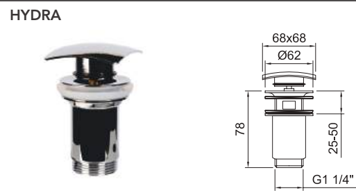
Válvula descarga sistema click-clack 1 1/4". Pop-up quick-clac 1 1/4".
