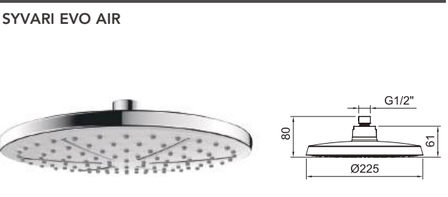
Rociador ducha Syvari Evo Air Ø225mm. Syvari Evo Air head shower Ø225mm.
