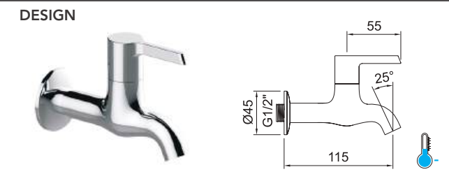
Grifo mural 1/2". Wall mounted tap 1/2".
